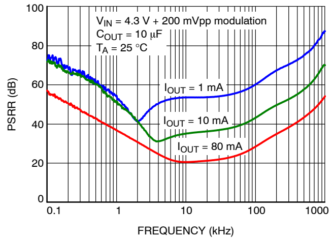
Figure 24. NCV8716x33xxx PSRR vs. Frequency
