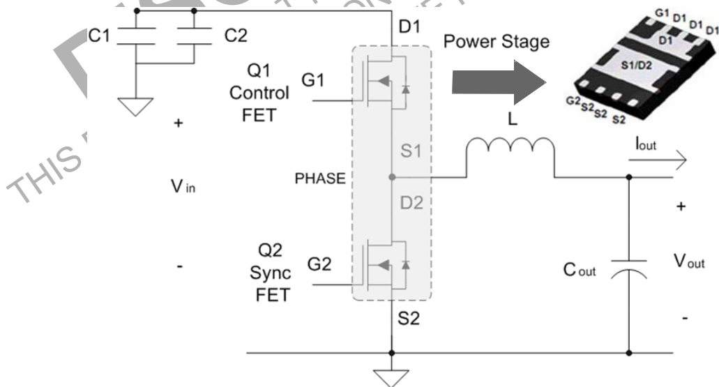
Figure 30. Shows the Power Stage in a Buck Converter Topology
