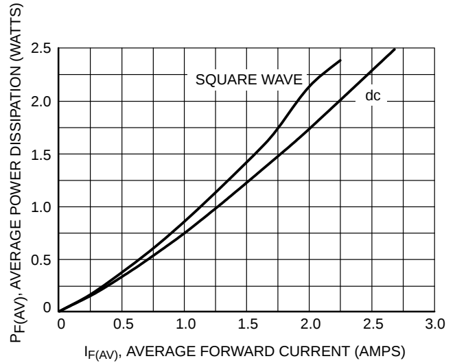
Figure 6. Power Dissipation
