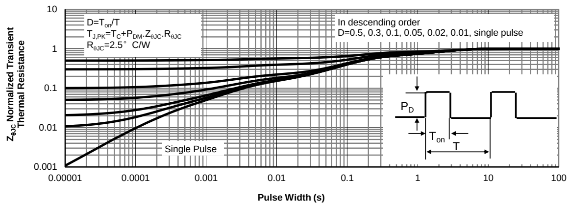
Figure 17: Normalized Maximum Transient Thermal Impedance for AOTF25S65 (Note F)
