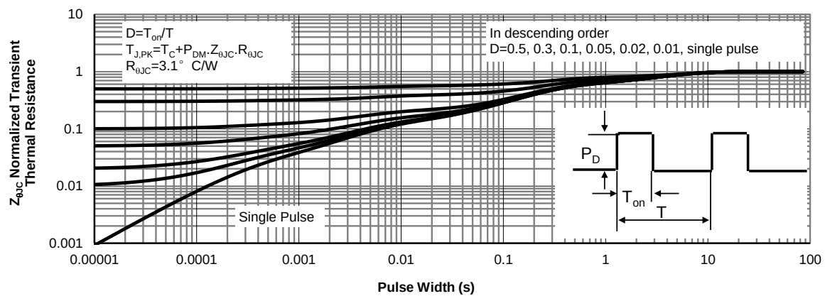
Figure 18: Normalized Maximum Transient Thermal Impedance for AOTF25S65L (Note F)
