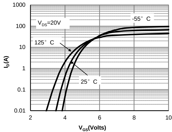
Figure 3: Transfer Characteristics
