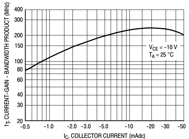
Figure 6. Current-Gain-Bandwidth Product
